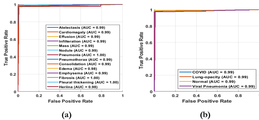
Figure. 4 ROC curve of proposed method for pulmonary disease classification, (a). CXR14 dataset(b). COVID-19 Radiography dataset
